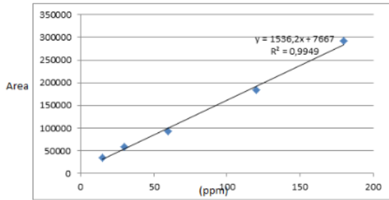
Fig.3. Liquiritin Standard Curve
