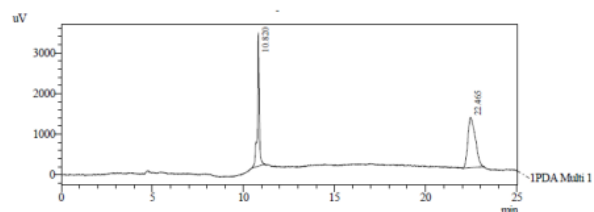
Fig.1. Pure Liquiritin Chromatogram Profile (RT 22.4 minutes) at 15 ppm Concentration Using HPLC.
